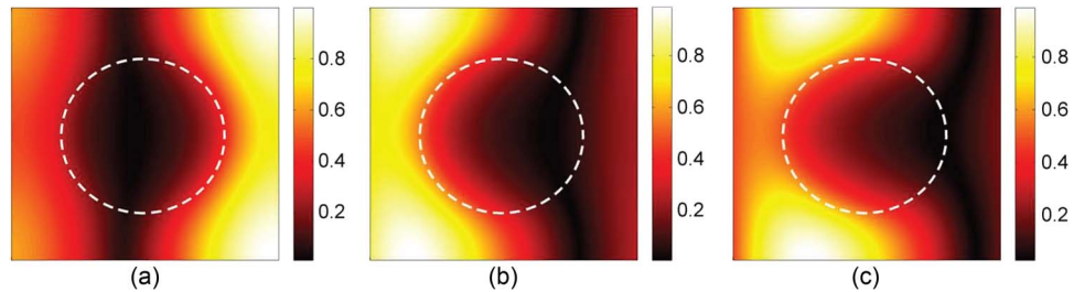
Fig. 7. E_z field distribution obtained by the proposed algorithm for TM_z mode with \text{Re}(\epsilon) + j\text{Im}(\epsilon) . (a) Normalized frequency 0.636 corresponding to the lower band edge. (b) Normalized frequency 0.701 corresponding to the bandgap. (c) Normalized frequency 0.774 corresponding to the upper band edge.
